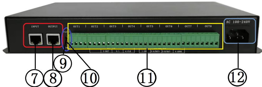
T-790K reverse view
