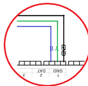
③. DMX512 single signal line wiring diagram ④. DMX512 differential signal wiring diagram (AB wire to write address)
