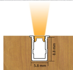
Slot Dimensions: 09(Depth) X 06(Width) mm
