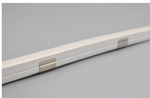
Stainless steel clip 20x10.8x8.4mm(LxWxH)
